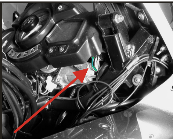
Splice switched relay wire to green wire with blue stripe.
